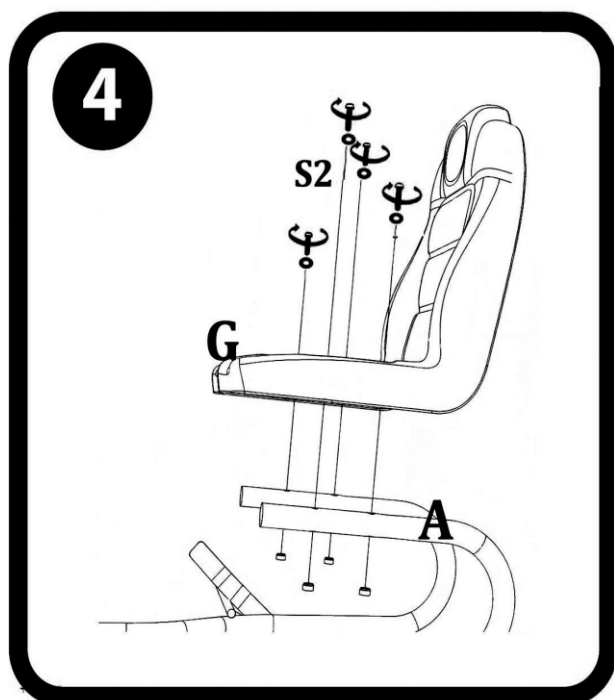
4. Seat assembly
