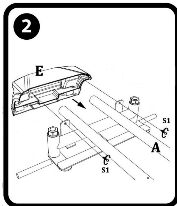
2. Front head part assembly
