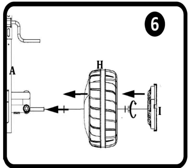
6. Front wheels assembly (2 sides)
