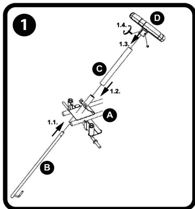
1. Steering pole + steering wheel assembly
