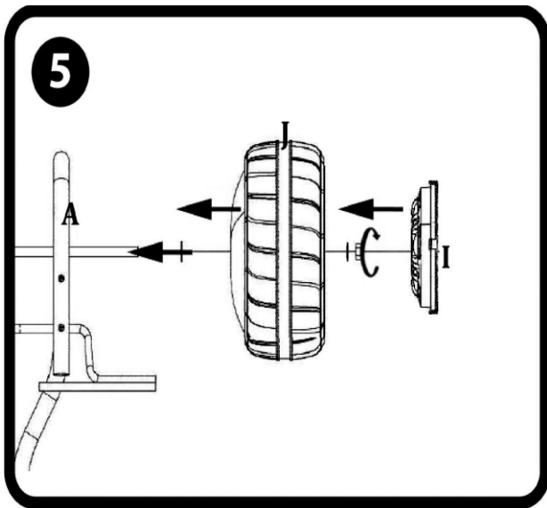
5. Rear wheels assembly (2 sides)
