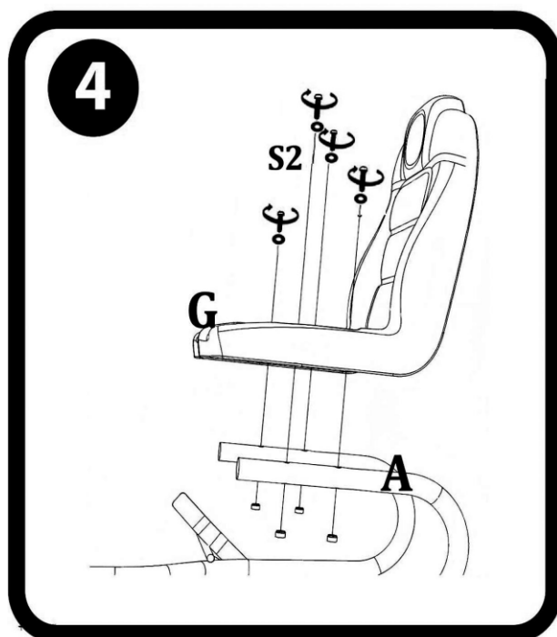
4. Seat assembly
