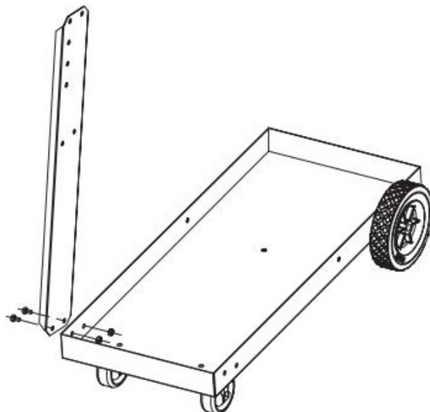
Figure C: Connection of Bottom Shelf and Left Support
