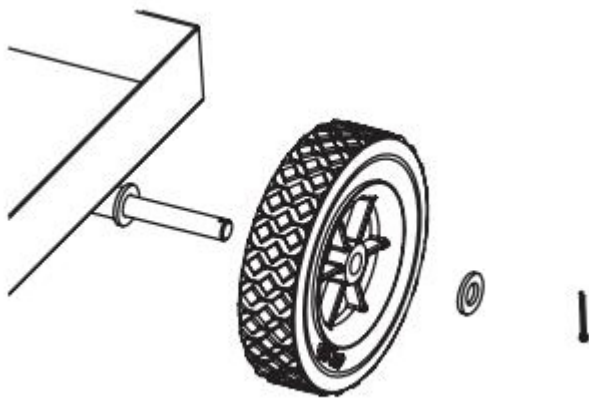
Figure A: Wheel Attachment
