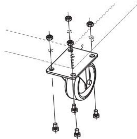
Figure B: Caster Attachment
